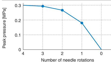
Peak pressure and the number of needle rotations (Supply pressure: 0.5 MPa)
